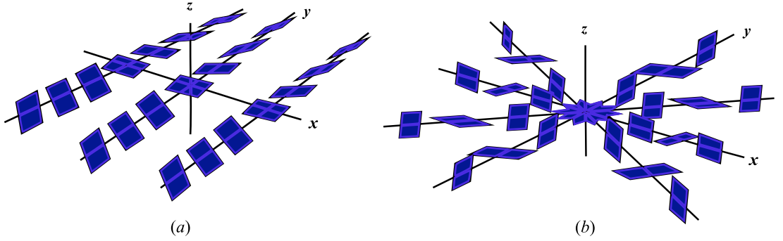
Figure 2.1: (a) The standard tight contact structure on \mathbb{R}^3 , (b) An overtwisted contact structure on \mathbb{R}^3 .
