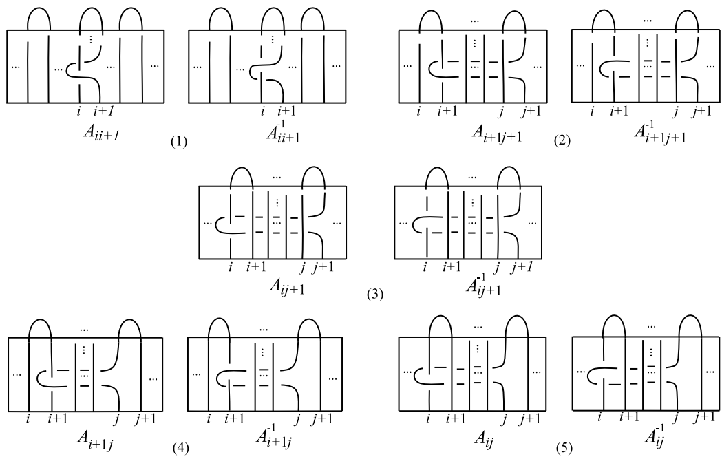
Figure 3.11: Generators: A_{ii+1}, A_{i+1j+1}, A_{ij+1}, A_{i+1j}, A_{ij} .
