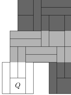
FIG. 5. A linked h -region P with four slices; leftmost slice Q is white, slices at distance 1 from Q are light gray, and slices at distance 2 from Q are dark gray.
