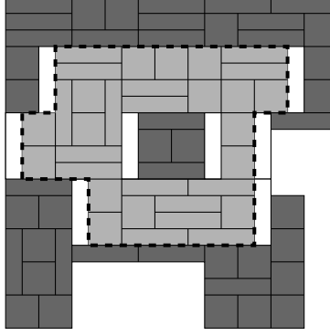
FIG. 7. A simply connected h -region G that is not an h/2 -region. Rectangles in S' are white, while region E' is shaded dark gray and region O' is light gray. The dashed line encloses h -region G' with strictly smaller area.
