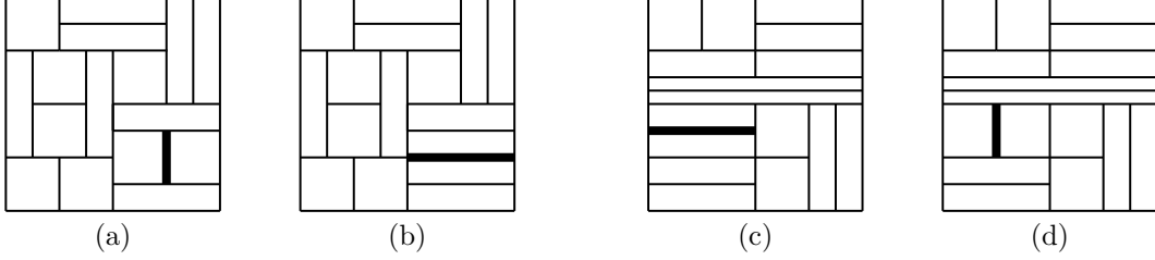
FIG. 3. Some tilings for n = 16 . Non-dyadic tilings (a) and (b) differ by an edge-flip. Dyadic tilings (c) and (d) differ by an edge-flip.
