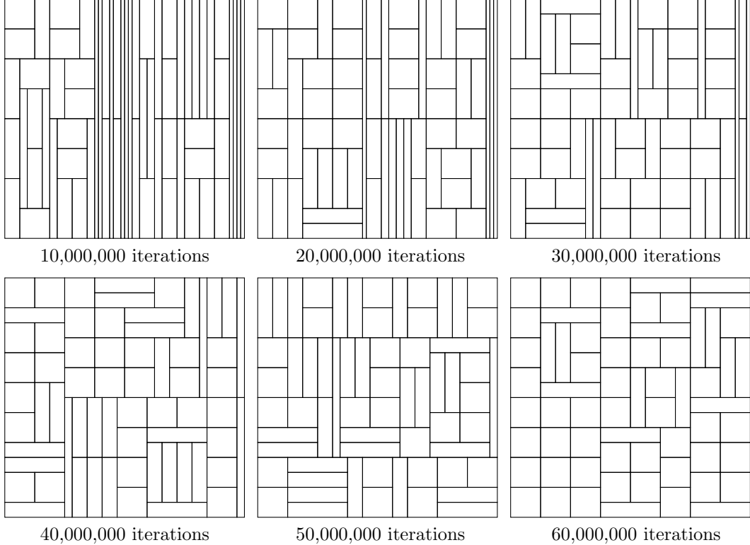
FIG. 15. A simulated execution of a Markov chain on \widehat{\Omega}_{64} with \lambda = 0.8 that includes both edge-flip moves and additional moves that select a random rectangular region and rotate the tiling within it by 180 degrees, starting with all vertical rectangles of width 1 and height 64.
