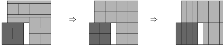
FIG. 9. An h -region P in which all connected components of E (dark gray) and O (light gray) are boundary h/2 -regions; the tiling of P after applying (1) to each; and the tiling of P by rectangles of height h resulting from edge-flips between vertically-adjacent rectangles of height h/2 .
