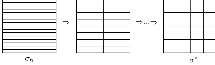
FIG. 10. A sequence of edge-flips from \sigma_h to \sigma^* .
