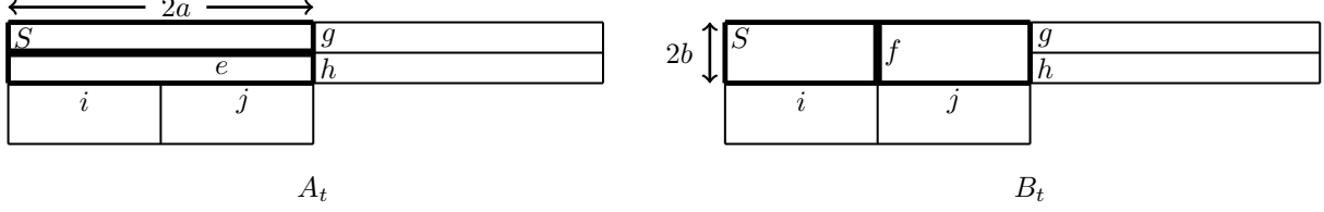
FIG. 12. An area 2n rectangle S bisected by horizontal edge e in A_t and vertical edge f in B_t . Four “bad” edge-flips g, h, i, j exist only if A_t and B_t are tiled in the neighborhood of S as shown.
