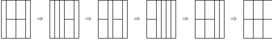
FIG. 8. The edge-flip sequence used to reduce the number of rectangles of height h given an interior h/2 -region tiled entirely by height h/2 rectangles.
