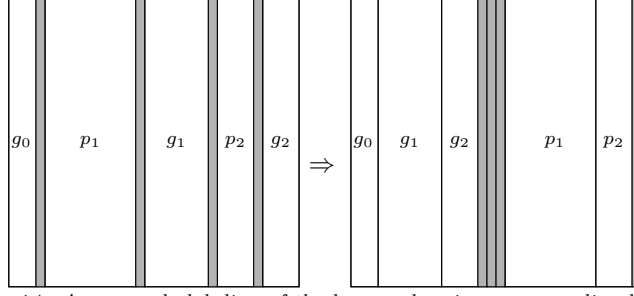
FIG. 14. An example labeling of the bars and regions surrounding bars.
