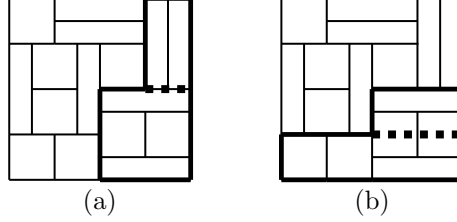
FIG. 4. For n = 16 , the bold lines in (a) define an 8-region that is not linked, while in (b) they give a linked 4-region. Slicing lines intersecting the interior of each region are dashed.
