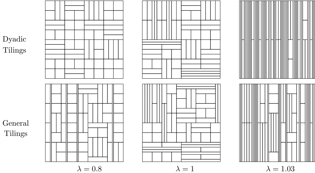
FIG. 2. \mathcal{M}_{64} and \widehat{\mathcal{M}}_{64} after 1,000,000 simulated steps for various values of \lambda , starting with all vertical rectangles of width 1 and height 64.
