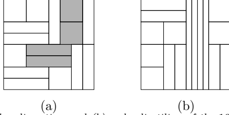
FIG. 1. (a) An equitable rectangular dissection and (b) a dyadic tiling of the 16 \times 16 square. Shaded rectangles are not dyadic.
