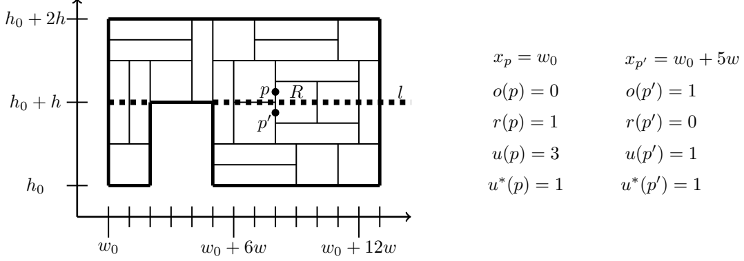
FIG. 6. An h -region P and a rectangle R crossing a slicing line illustrating the definitions r(p) , o(p) , u(p) , and u^*(p) .
