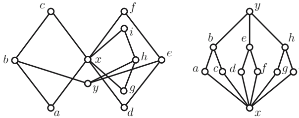
Fig. 3 A non-planar poset with a planar cover graph
