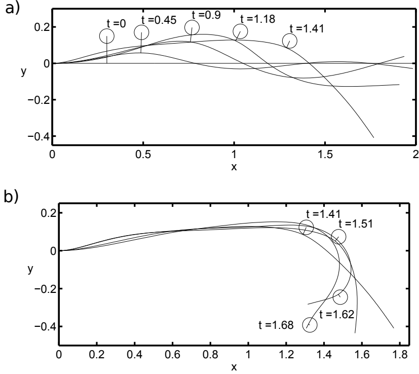
FIGURE 6. Vortex-filament dynamics for R_2 = 0.01 , x_0 = 0.3 , y_0 = 0.15 . Snapshots of the filament and point vortex (circle), with line segments connecting the two at corresponding times (shown adjacent to the point vortex). a, Up to t = 1.41 . b, From t = 1.41 on.
