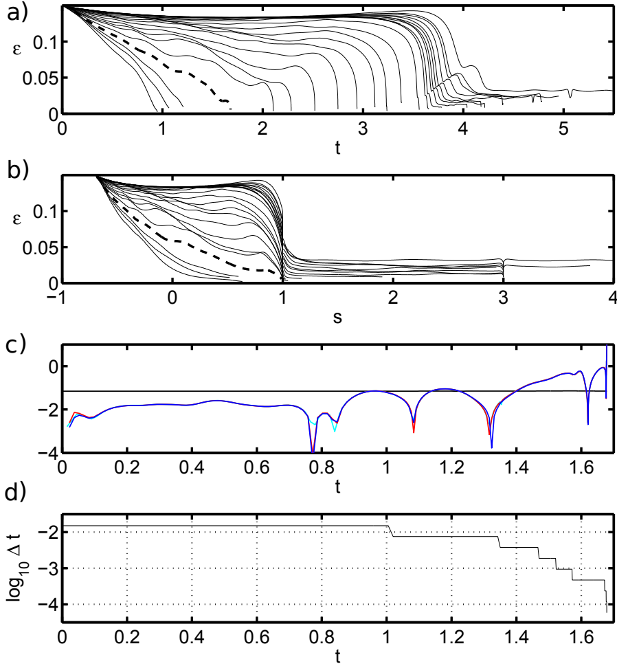
FIGURE 7. Separating distances, energy fluxes, and time step during approaches of vortices to filaments. a, The minimum distance from the vortex to the filament ( \epsilon ), versus time, for filaments with 24 different values of R_2 ranging over three orders of magnitude. The values are 0.0042, 0.006, 0.0075, 0.01, 0.014, 0.02, 0.024, 0.03, 0.042, 0.06, 0.075, 0.1, 0.14, 0.2, 0.24, 0.3, 0.42, 0.6, 0.75, 1, 1.4, 2, 2.4, and 4.2. In each case x_0 = 0.3 , y_0 = 0.15 . b, The values of \epsilon from ‘a’ now plotted with respect to the arc length location on the filament nearest to the vortex. The arc length is continued above 1 as the vortex travels around the free end of the filament. c, For R_2 = 0.01 , the dashed lines in ‘a’ and ‘b’, values of total energy and energy fluxes versus time. The horizontal line is \log_{10} |\widetilde{K}E_{fluid} + U_{el}| (fluid kinetic energy plus elastic energy). The curved lines show \log_{10} |d\widetilde{K}E_{fluid}/dt| (red line), \log_{10} |dU_{el}/dt| (dark blue line), and \log_{10} |P| (light blue line) (the rates of change of fluid kinetic energy and elastic energy, and the rate of work done by the filament on the fluid). d, For R_2 = 0.01 , the logarithm, base 10, of the time step, versus time.
