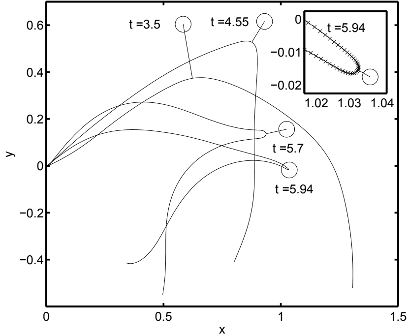
FIGURE 9. Snapshots of point vortex and filament for R_2 = 10^{-5} , y_0 = 0.5 , x_0 = 0.3 . The inset shows a close-up near the vortex, and the spatial grid on the filament, at the final time.
