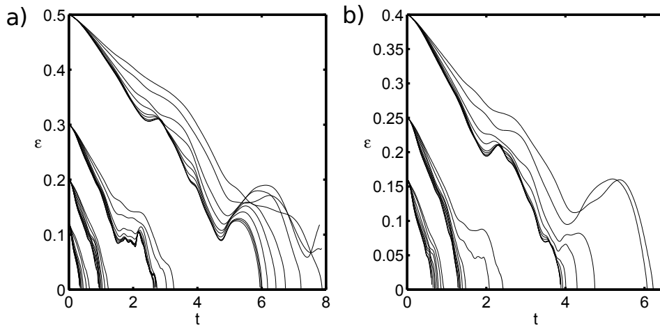
FIGURE 8. a, Vortex filament distance versus time for y_0 = 0.12, 0.2, 0.3, and 0.5 , and ten values of R_2 : 1,2,3 \times 10^{-5} , 1,2,3,6 \times 10^{-4} , and 1,2,3 \times 10^{-3} . In all cases, x_0 = 0.3 . b, Same data as in ‘a’ but for y_0 = 0.16, 0.25, and 0.4 .
