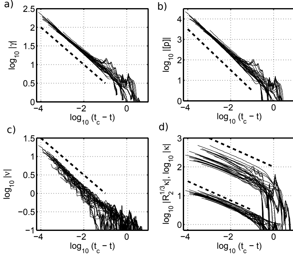
FIGURE 13. \log_{10} |\gamma| , \log_{10} |[p]| , \log_{10} |\nu| , and \log_{10} |\kappa| at the point on the filament nearest to the vortex, for the simulations corresponding to data from 30 of the 70 curves in figures 8 and 12, with the same \log_{10}(t_c - t) values as in figure 12. For the |\kappa| data, the lower set of curves, below the lower dashed line, shows \log_{10} |R_2^{1/3} \kappa|
