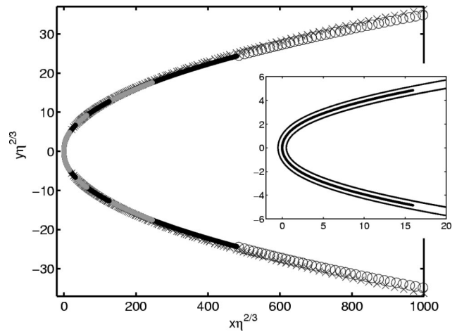
FIG. 11. Convergence of numerical fiber shapes and streamlines to a quasiseparabolic universal shape. Shown in alternating shades are the fiber shapes for \eta=200, 550, 1500, 4050, 11000, and 30000 , as well as the streamlines for the smallest and largest values (crosses and circles, respectively), with x and y scaled by \eta^{2/3} . The asymptotic parabola has the form Y=1.11X^{1/2} . (Inset) Numerical fiber shapes for \eta=200 (thin black line), 4050 (white line), and 30000 (thick black line) in the tip region, where the universal shape fits the parabola Y=1.34X^{1/2} .
