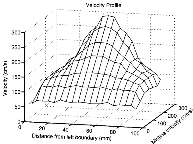
FIG. 4. The background velocity profile of the soap film, shown as a function of the velocity at the midline, and measured in the absence of the fiber. Each panel extends over 0.5 cm horizontally. Thus the longest fiber in Fig. 3(b) (5.15 cm) occupies five segments to either side of the vertical center line in its undeflected state. At the highest flow speed used in Fig. 3(b) (270 cm/s) its profile width is less than 2 cm, so it lies within two segments to either side of the center line.
