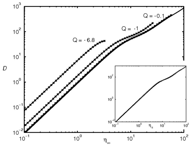
FIG. 17. Drag vs \eta_\infty for Riabouchinsky solutions with Q = -6.84, -1, -0.1, and 0 (Helmholtz) moving from left to right. For each Q the data are shown for the maximum intervals in which the solutions exist. (Inset) Drag vs \eta_s for the same solutions.
