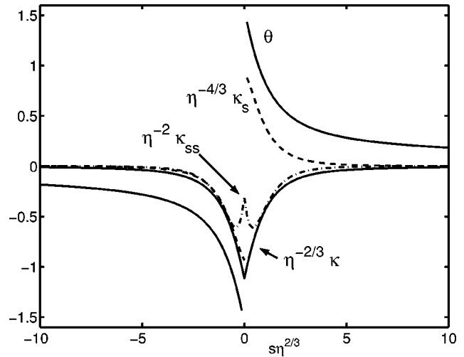
FIG. 9. The asymptotic form of the rescaled numerical solutions near the tip as \eta \rightarrow \infty , in terms of \theta (solid lines), \eta^{-2/3}\kappa (solid line), \eta^{-4/3}\kappa_s (dashed line), and \eta^{-2}\kappa_{ss} (dashed-dotted line). The first and third functions are antisymmetric and the second and fourth are symmetric about s\eta^{2/3} = 0 .
