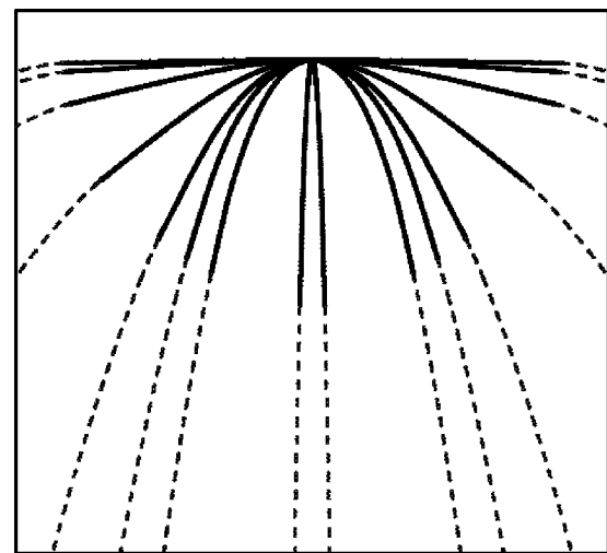
FIG. 6. Fiber shapes for a range of \eta . The solid lines are the fibers and the dashed lines are the free streamlines. The solutions shown correspond to \eta=1, 2, 4, 8, 16, 32, 64 , and 30 000, increasing from flat to folded-over. A measure of the transition is d\theta_{\text{end}}/d\eta , the rate of change of the tangent angle at the fiber end with respect to \eta , which peaks at \eta=5.6 .
