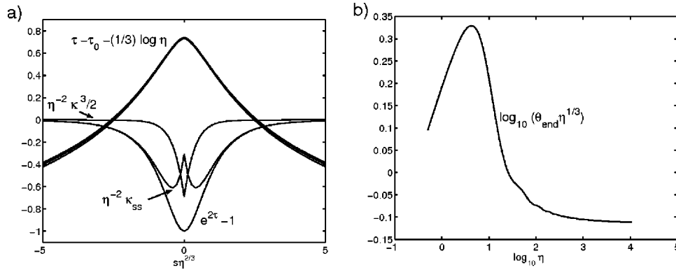
FIG. 10. Tip and end region behavior of numerical solutions. (a) Convergence of \tau - \tau_0 - (1/3)\log \eta to a constant C at the tip. Also shown is the convergence of the normalized pressure loading e^{2\tau} - 1 = \eta^{-2}[\rho] , and the two elastic terms \eta^{-2}\kappa_{ss} and \eta^{-2}\kappa^{3/2} which sum to it in the force balance. Note that the cubic elastic term decays more rapidly than the \eta^{-2}\kappa_{ss} term, which holds outside of the tip region as well. (b) Numerical evidence for the convergence of the tangent angle at the end of the fiber, normalized by \eta^{1/3} , to a constant C_0 as \eta \rightarrow \infty . This implies that the universal fiber shape is quasiparabolic. The peak of the curve occurs near the transition to bending.
