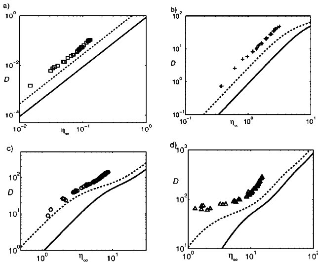
FIG. 15. The choked-flow drag curves (lines covered by small symbols) compared to the Helmholtz drag curve (solid line) and the four sets of experimental data shown in Fig. 3(b). (a) H=9/1.95 , corresponding to the most rigid fiber ( E=2000 ) used in the experiment; (b) H=9/1.79 , E=2.8 ; (c) H=9/3.3 , E=2.8 ; and (d) H=9/5.15 , E=2.8 .
