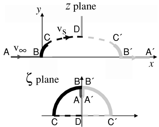
FIG. 16. The symmetric Riabouchinsky flow domain in the z and \zeta planes. The ordinate I_0 of A is a free parameter set by the wake pressure Q .
