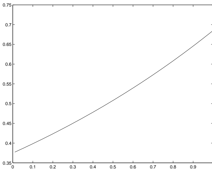
Figure 4 - Behavior of the ratio E_M(t)/E_W(t) with respect to the time for 0 < t \leq 1
