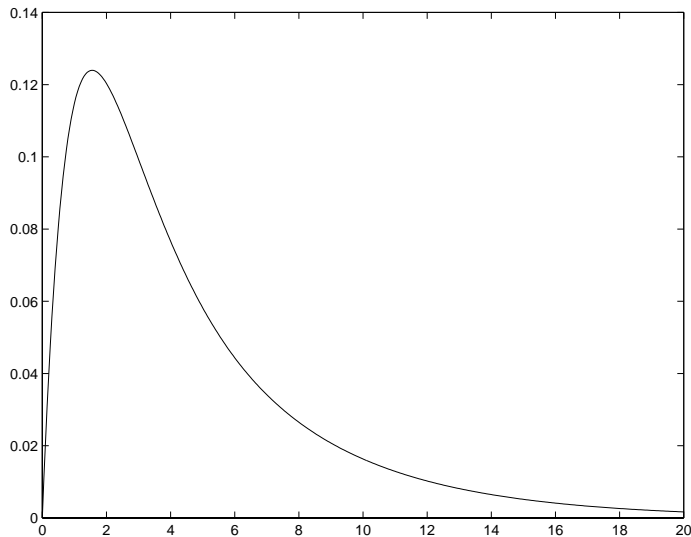
Figure 1 - Behavior of E_M(t) with respect to the time for 0 \leq t \leq 20
