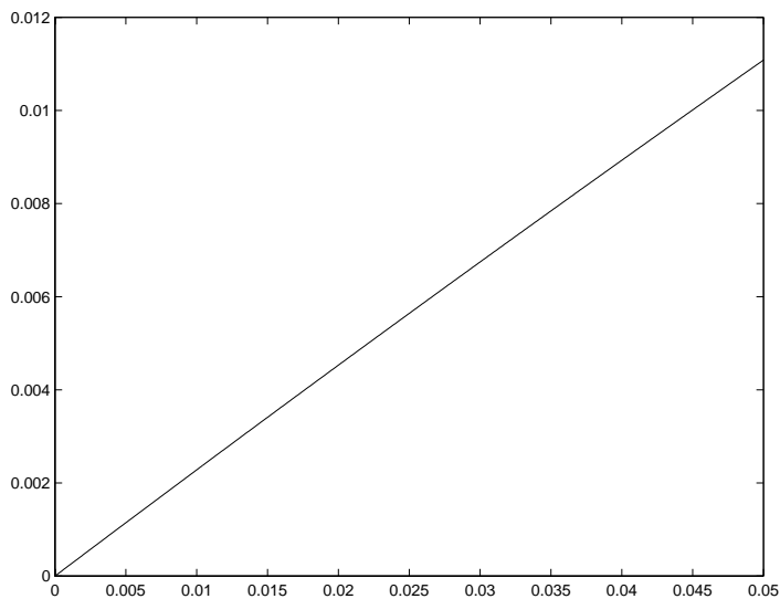
Figure 2 - Detail of Figure 1 for small times
