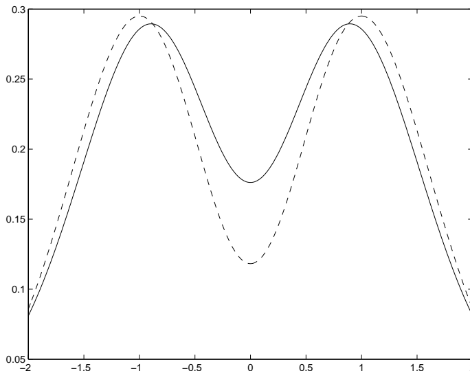
Figure 3 - Comparison between the exact solution f_E (dashed line) and its approximation f_E^{(1)} (continuous line) with the method of moments for t = 1
