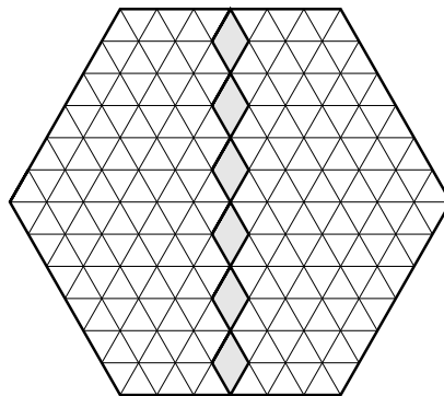
FIGURE 1.10.
