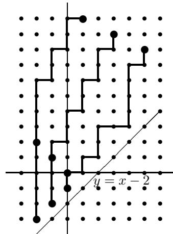
FIGURE 2.3(b).
