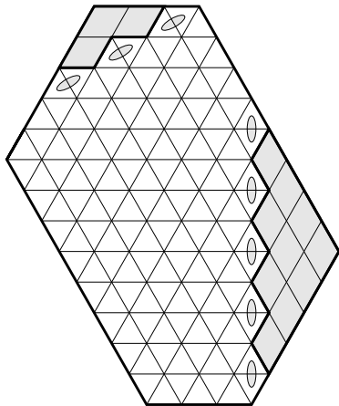
FIGURE 1.3(c). H_d(5, 3, 8) .
