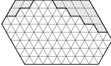
Figure 1.6. H_a(3, 8, 5) .
