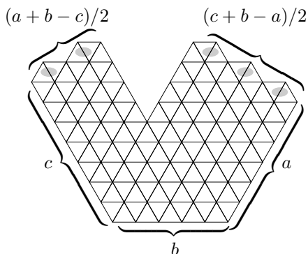
FIGURE 1.7(b). H_n(6, 5, 7)
