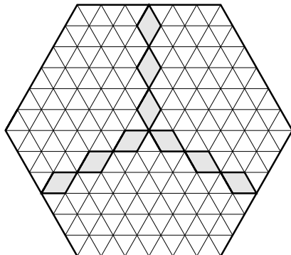
FIGURE 1.11.
