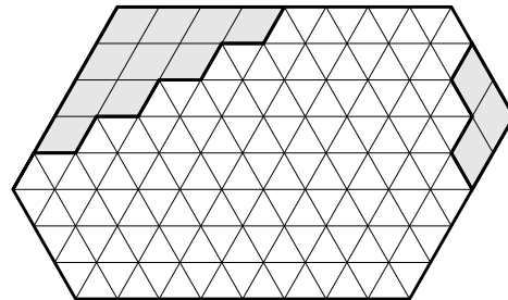
FIGURE 1.3(d). H_d(5, 8, 3) .
