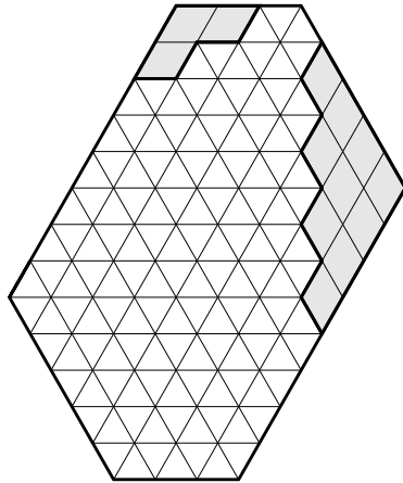
FIGURE 1.3(a). H_d(8, 3, 5) .
