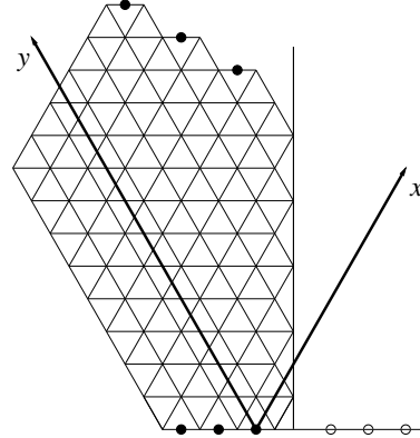
FIGURE 2.7.
