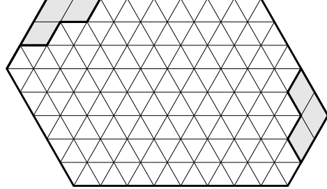
FIGURE 1.3(f). H_d(3, 8, 5) .
