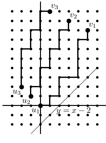
FIGURE 2.3(a).
