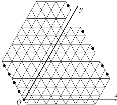
Figure 2.5. R(5, 10, (7, 6, 4, 2, -1)) .
