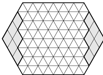
Figure 1.8. H_o(4, 6, 4) .
