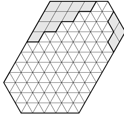
FIGURE 1.3(b). H_d(8, 5, 3) .
