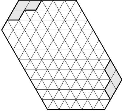
FIGURE 1.3(e). H_d(3, 5, 8) .
