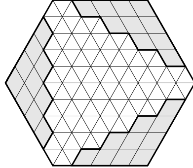
FIGURE 1.5. T_5 .
