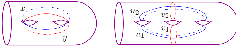
FIGURE 2. Left: The curves x and y form a symmetric simply intersecting pair. Right: the curves u_1, v_1, u_2 , and v_2 form a symmetrized simply intersecting pair.
