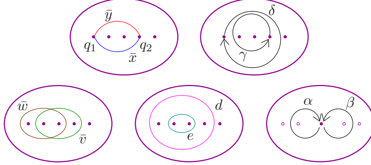
FIGURE 7. Curves, loops, and arcs used in the second proof of Theorem 3.1
