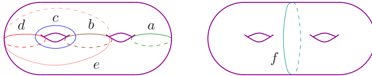
FIGURE 5. The curves a, b, c, d, e , and f from Theorem 2.1.
