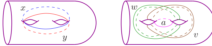
FIGURE 6. The curves used in Theorem 3.1.
