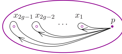
FIGURE 4. The generators x_i for \pi_1(D_{2g-1}^\circ) .
