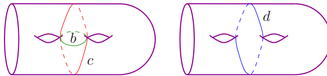
FIGURE 3. The curves used to define Johnson's mapping class.
