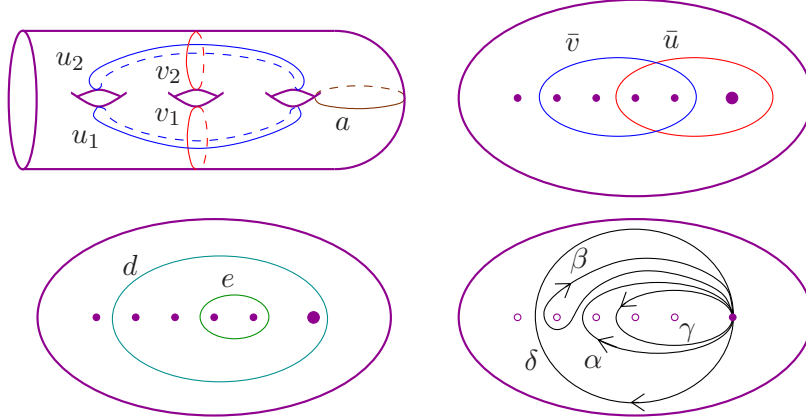
FIGURE 8. The curves and loops used in the proof of Theorem 3.2.
