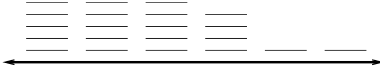
FIGURE 7. A linear (4, 15) -society with n = 21 voters. Here q = 4 and \rho = 2 , so the clique number is at least \lceil (n - \rho)/q \rceil = 5 .
