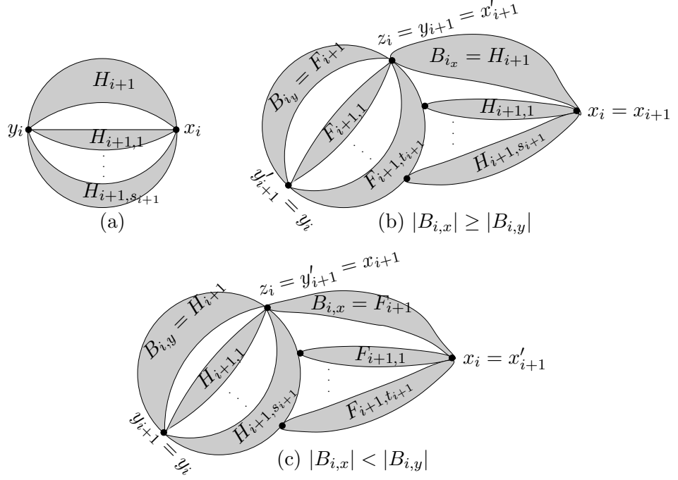
Figure 4: The descriptions of (R1) and (R2).
