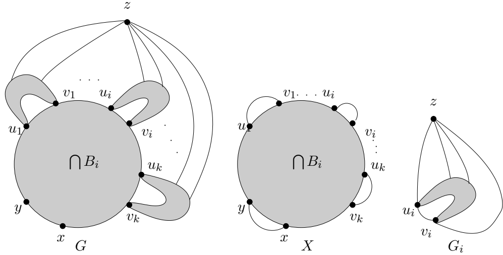
Figure 3: The description of \mathcal{U} = \{\{u_1, v_1\}, \dots, \{u_k, v_k\}\} , X and G_i .
