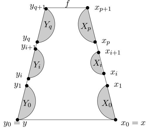
Figure 5: The blocks X_0, \dots, X_p and Y_0, \dots, Y_q .
