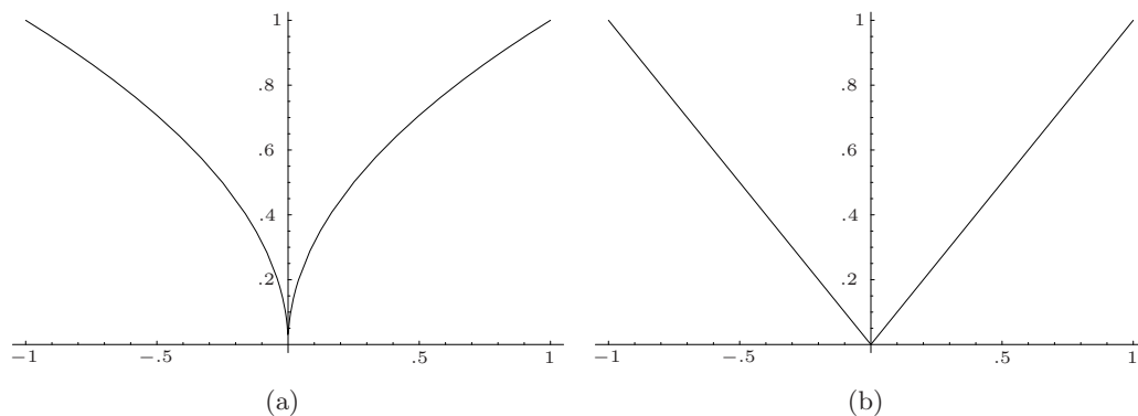
Figure S1. Illustration of the difference among continuous, locally Lipschitz, and differentiable functions. (a) shows the graph of f : \mathbb{R} \rightarrow \mathbb{R} , f(x) = \sqrt{|x|} , which is continuous at 0, but not locally Lipschitz at 0. (b) shows the graph of f : \mathbb{R} \rightarrow \mathbb{R} , f(x) = |x| , which is locally Lipschitz at 0, but not differentiable at 0.
